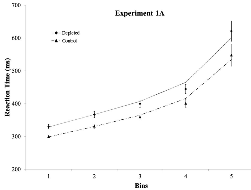
Figure 3. Vincentile plots for depleted and control conditions for the first quartile of Phase 2 in Experiment 1A. Mean vincentiles are represented by data points and standard error bars, whereas the best fitting ex-Gaussian vincentiles are represented by lines.
