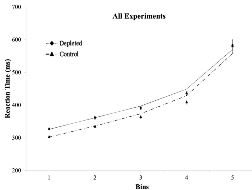
Figure 7. Vincentile plots for depletion and control groups (in the no-motivation condition only) collapsed across all experiments. Mean vincentiles are represented by data points and standard error bars, whereas the best fitting ex-Gaussian vincentiles are represented by lines.
