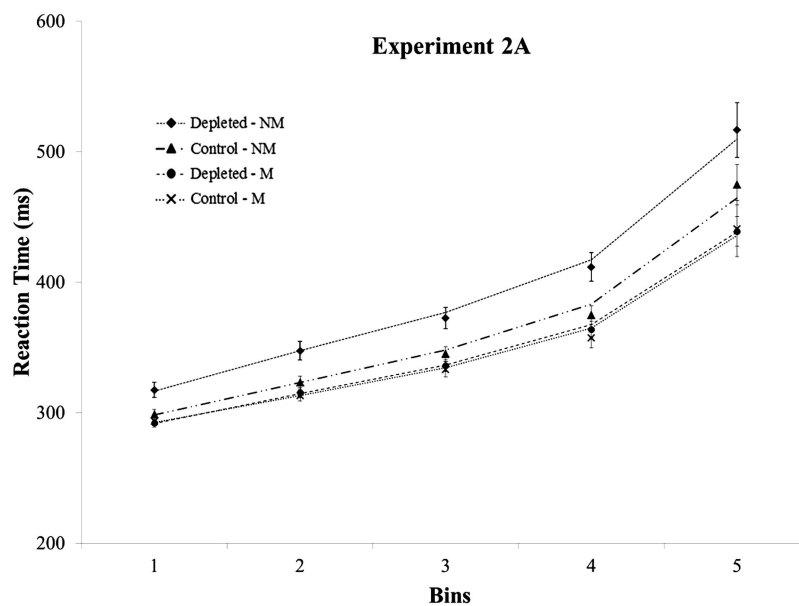
Figure 5. Vincentile plots for depleted and control groups in both the motivation (M) and no-motivation (NM) groups for the first quartile of Phase 2 in Experiment 2A. Mean vincentiles are represented by data points and standard error bars, whereas the best fitting ex-Gaussian vincentiles are represented by lines.
