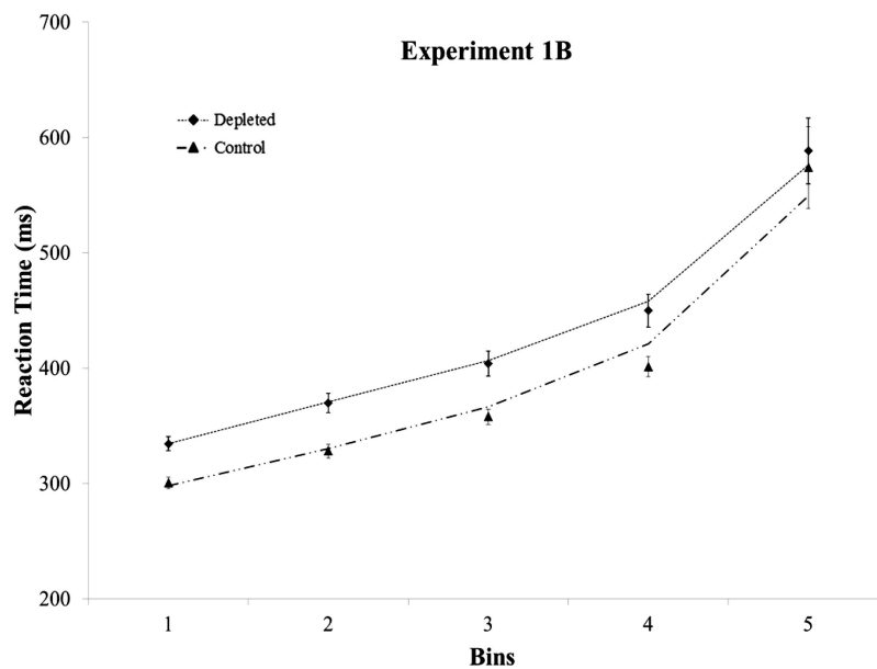
Figure 4. Vincentile plots for depleted and control conditions for the first quartile of Phase 2 in Experiment 1B. Mean vincentiles are represented by data points and standard error bars, whereas the best fitting ex-Gaussian vincentiles are represented by lines.
