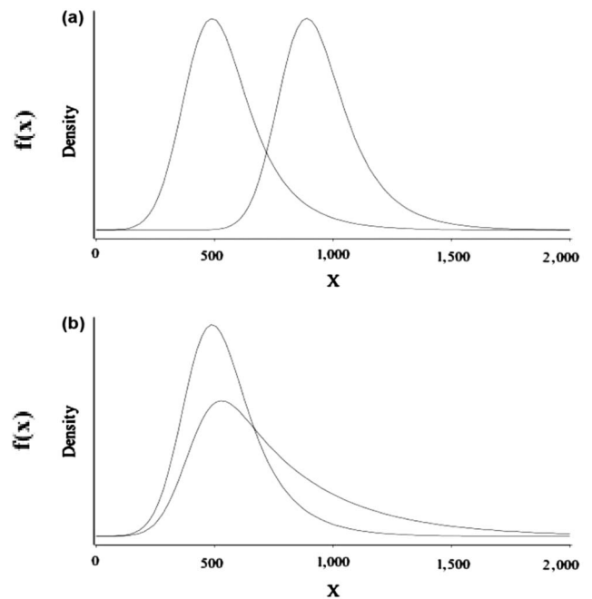
Figure 1. (a) Two hypothetical ex-Gaussian distributions with changes in \mu only. (b) Two hypothetical ex-Gaussian distributions with changes in \tau only.
